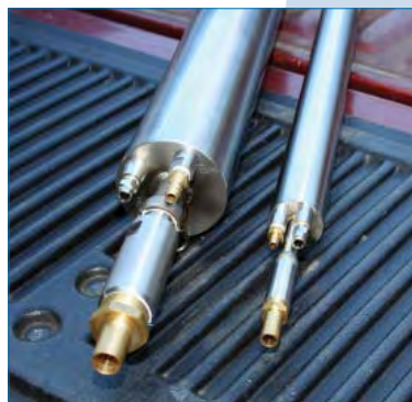
Top view of TR-975 and TR-977 bottom-loading pumps
