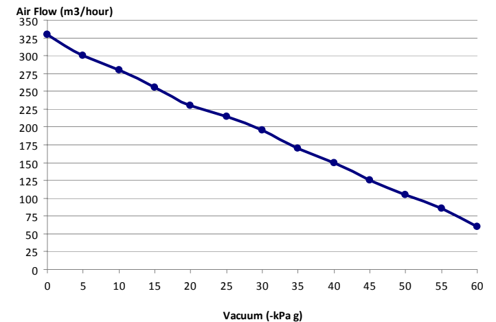
Pilot Unit Performance With Cooling System and GAC in Exhaust Stream
